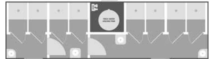
FLOOR PLAN
